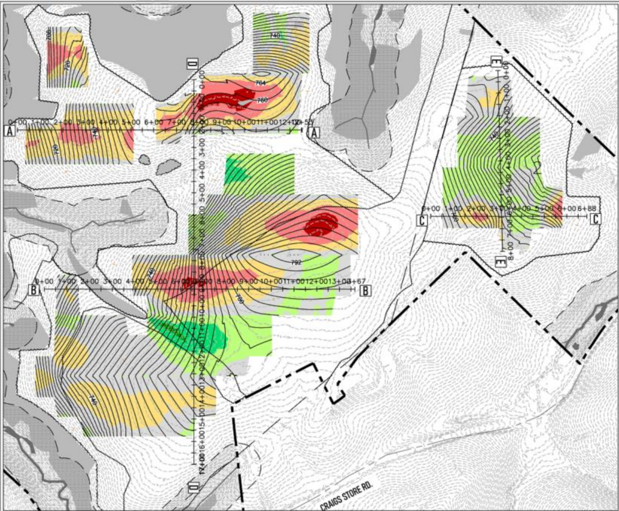
CUT/FILL MAP NTS
